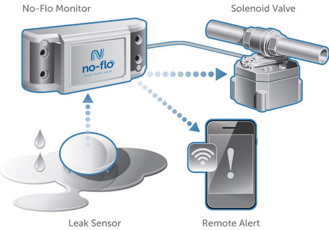
The No-Flo Leak Sensor is an integral part of the No-Flo smart water cut off system
